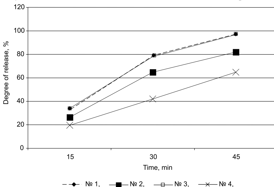
Fig. 1. Kinetics of gylsulphazide release.
